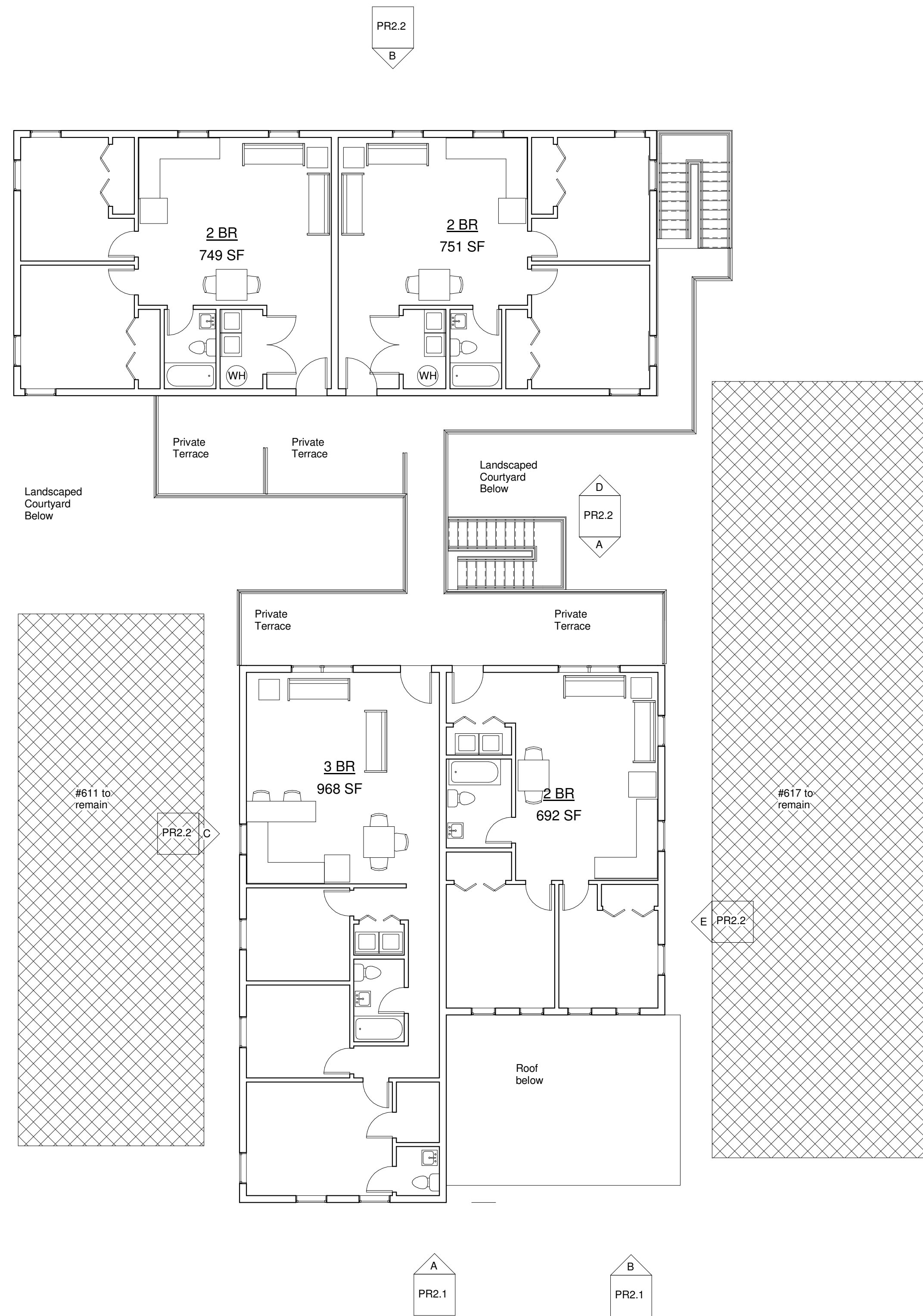
1 Schematic Level 3 Plan 1/8" = 1'-0"
